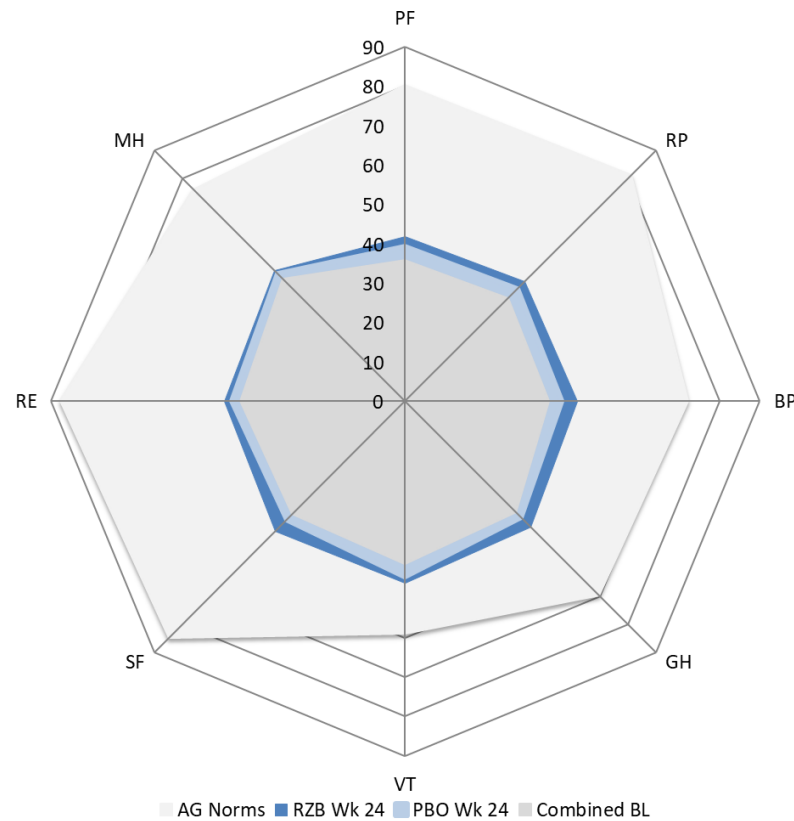
Supplemental Figure 1. Syndergram Visualization of Differences between Patients Receiving Risankizumab versus Placebo in SF-36 Domains at 24 Weeks
