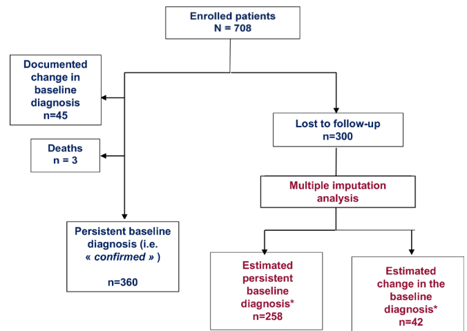
Figure 1 Flow chart of 708 patients with recent low back pain considered as having axSpA, over their 10-year follow-up in the Devenir des Spondyloarthrites Récentes (DESIR) cohort. *See the Methods section. We considered a patient as 'estimated change in the baseline diagnosis' in case a change in diagnosis was estimated in at least 7 out of the 10 imputed datasets. axSpA, axial spondyloarthritis.
