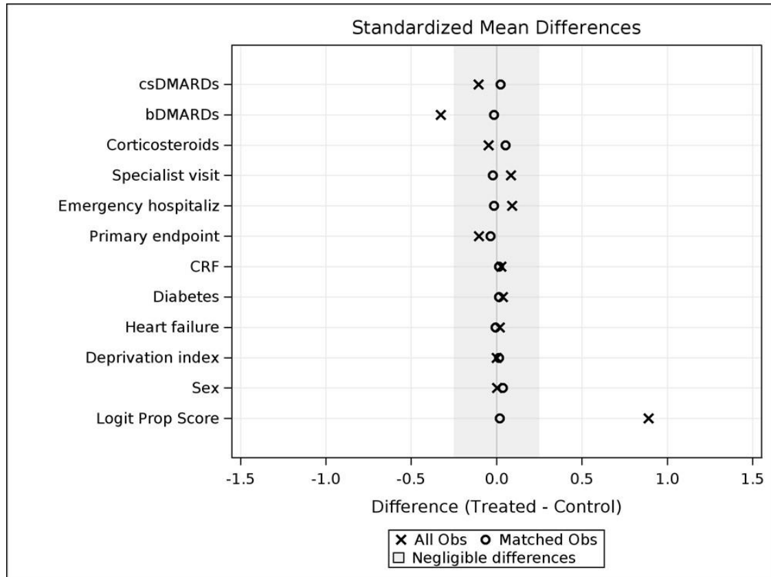
Supplementary Figure 1. Comparison before (all observations) and after use of propensity score (matched observations).
