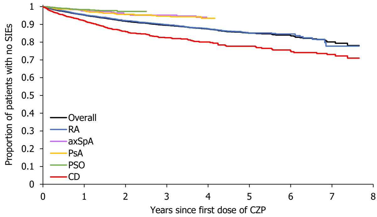
A. Kaplan-Meier graph of time to first expert-confirmed SIE: 0–8 years exposure
