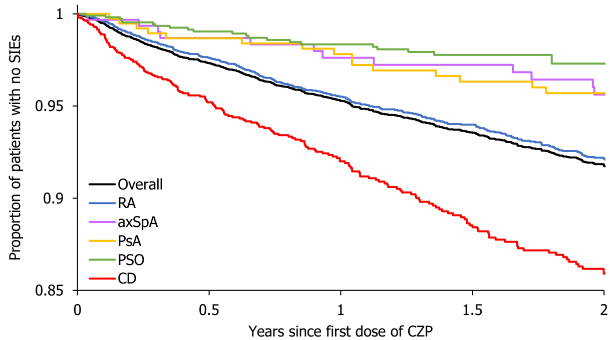
B. Kaplan-Meier graph of time to first expert-confirmed SIE: 0–2 years exposure (taken from panel A)
