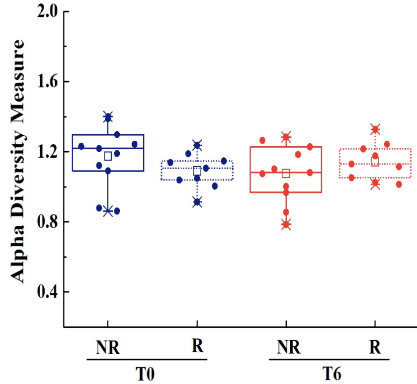
Determination of the Alpha Diversity at the Order level using the Shannon-Weiner index:
