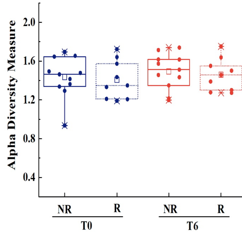
Determination of the Alpha Diversity at the Family level using the Shannon-Weiner index:
